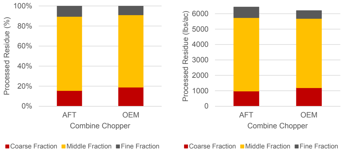
Figure 37. Comparison of the average residue distribution fractions between OEM and AFT choppers as a percentage (left) and density (right).
